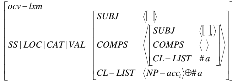
Figure 17. Object-control verb after cliticization
