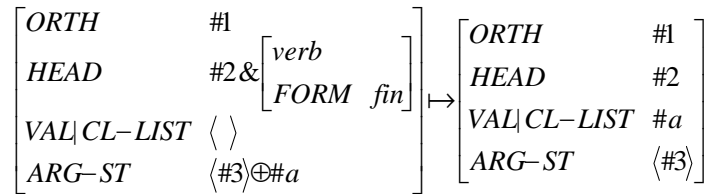
Figure 5. Simple cliticization rule
