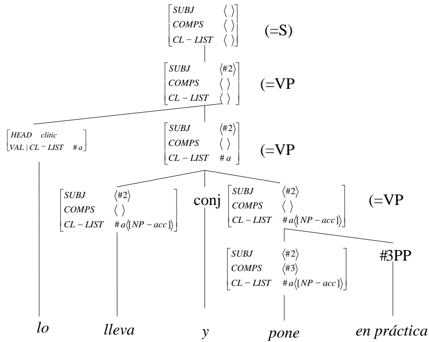
Figure 24. Analysis of clitic coordinated sentence
