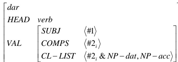
Figure 26. Doubled cliticized lexeme
