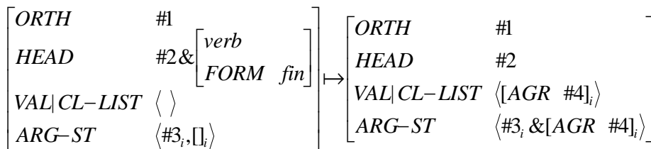
Figure 28. Lexical rule for the direct reflexive
