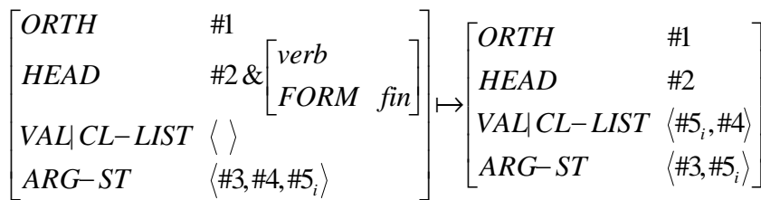
Figure 25. Lexical rule for duplication of the cliticized complement
