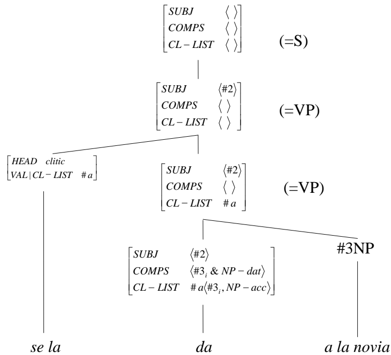
Figure 27. Analysis of clitic sentence with duplication of arguments
