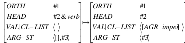
Figure 31. Lexical rule for the passive-reflexive
