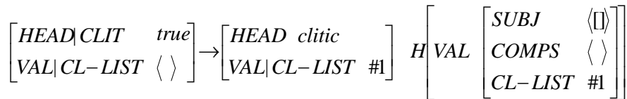
Figure 6. Head Proclitic Rule
