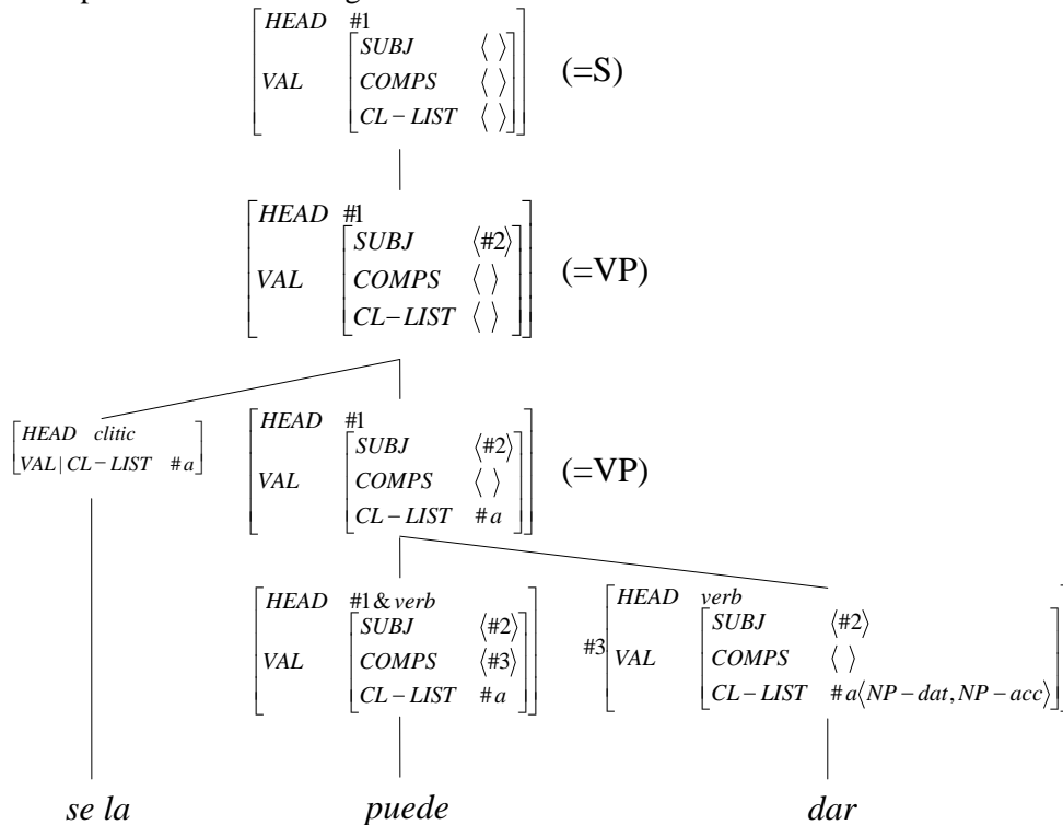
Figure 9. Analysis of simple clitic climbing
